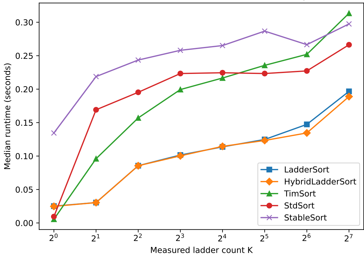
Runtime vs measured K, randomized exact-K interleaving, N=1000000
